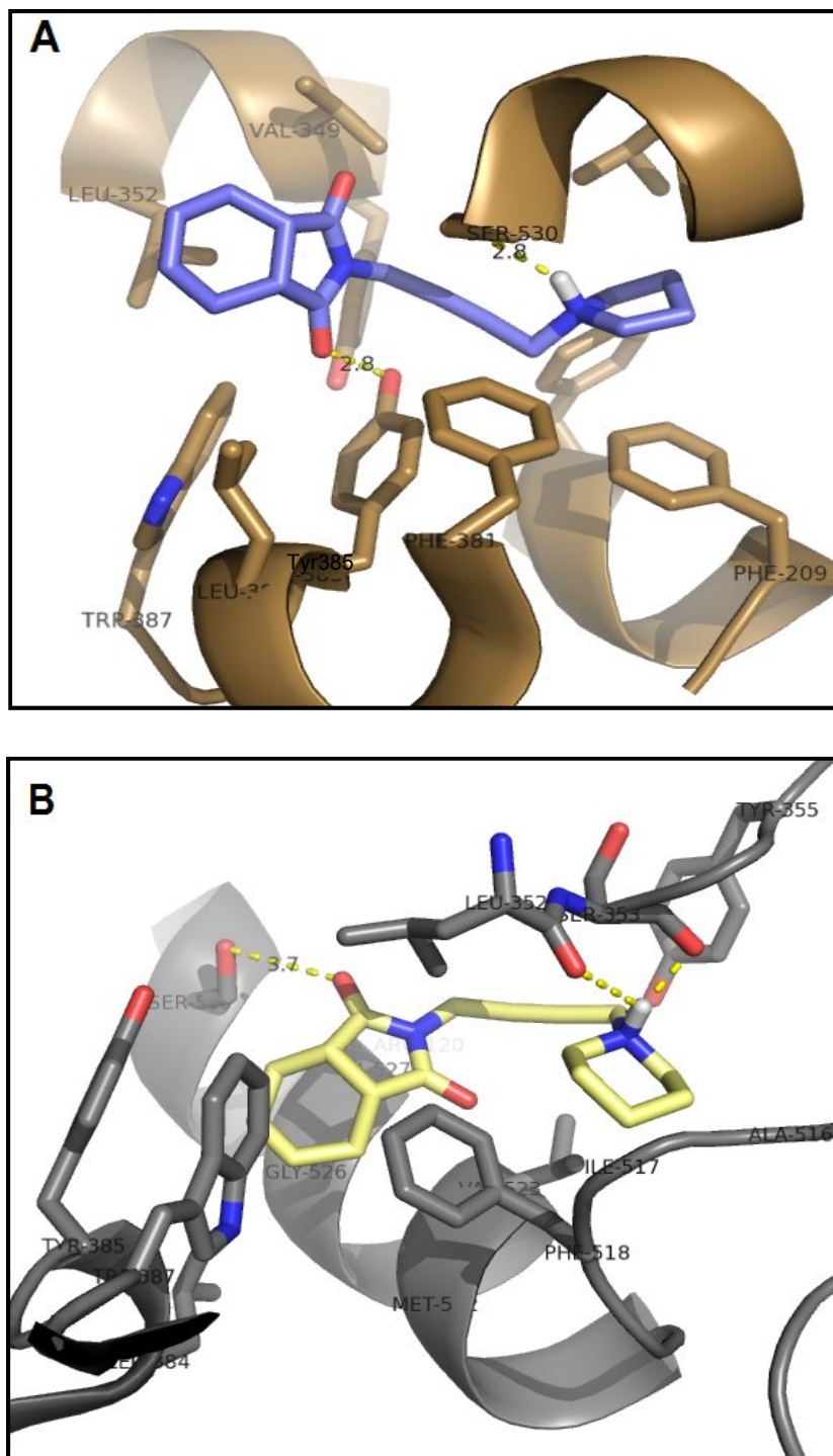
Figure 4.2. (A) Binding mode of Am6 (blue) within the COX-1 active site (gold). (B) Binding mode Am4 (yellow) within the COX-2 active site (gray), respectively. Yellow dotted lines indicate for hydrogen bonding.
